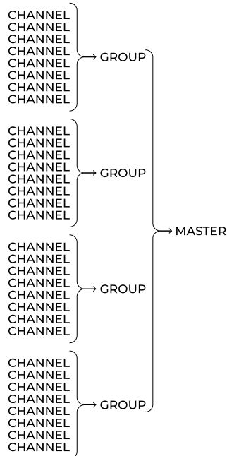
Figure 18: CGM structure.
