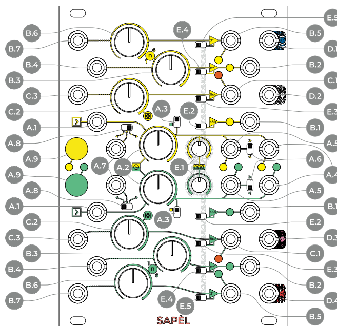
Figure 28: SAPÈL interface.
