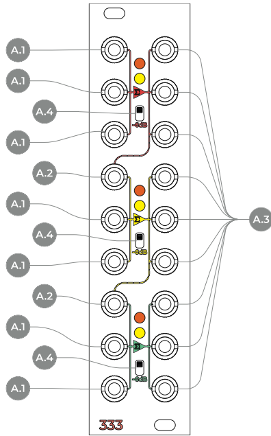
Figure 103: 333 interface.
