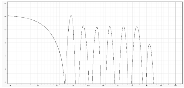
Figure 40: Odd bands output, detail.
