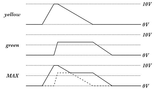
Figure 48: AHDSR envelope with FALISTRi's Quadrature .
