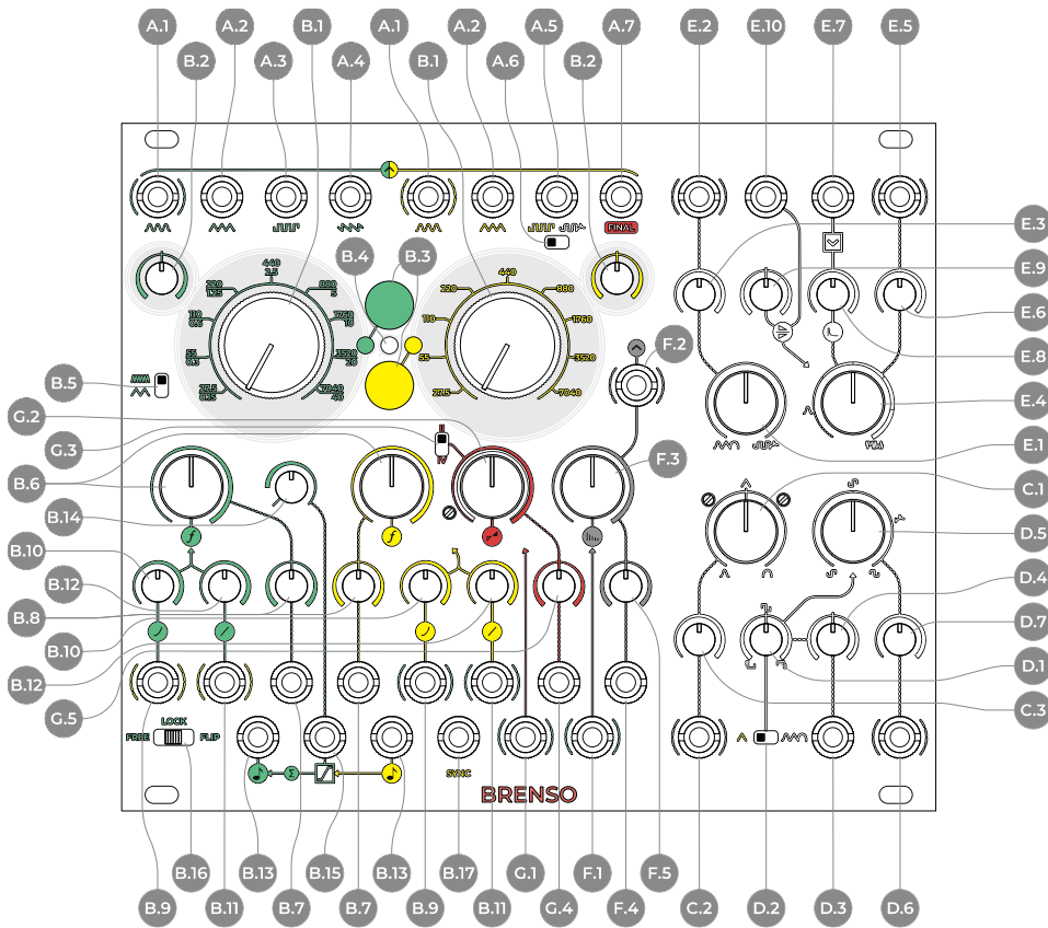
Figure 95: BRENDO interface.
