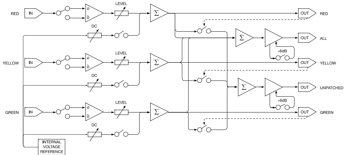
Figure 106: 321 flow chart.
