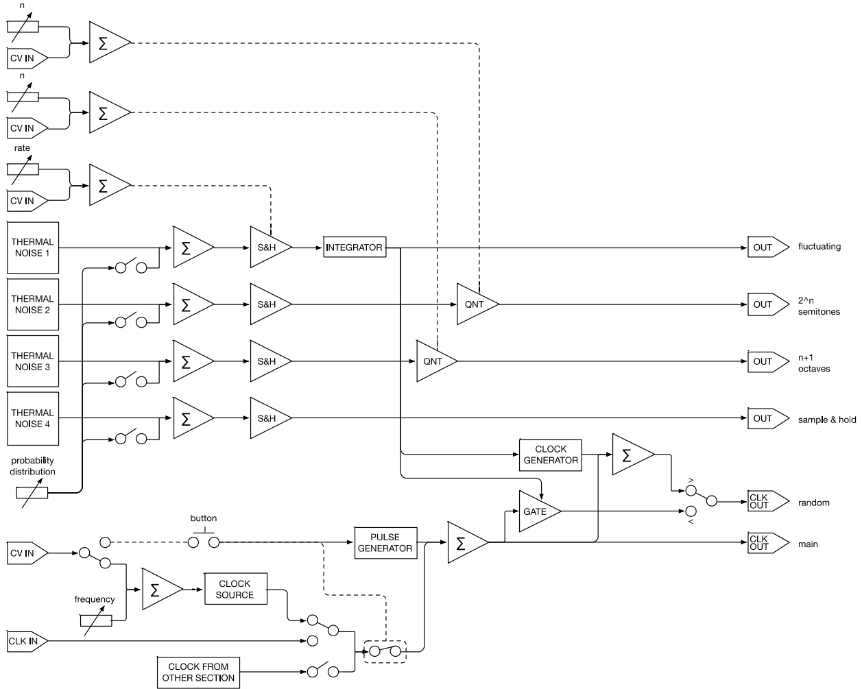
Figure 31: SAPÈL's flow chart.
